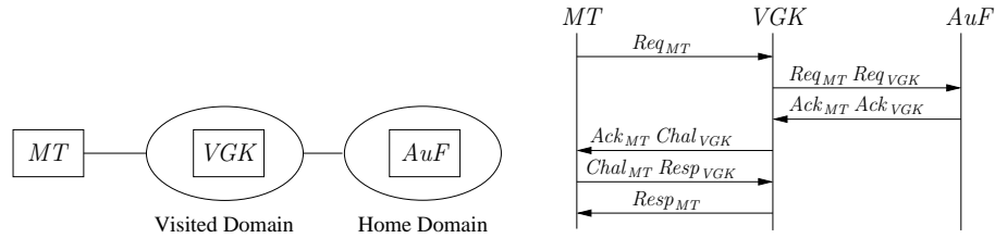
Fig. 2. The H.530 protocol (simplified). The deployment of the protocol is on the left, the messages exchange between the participants are summarized on the right.
